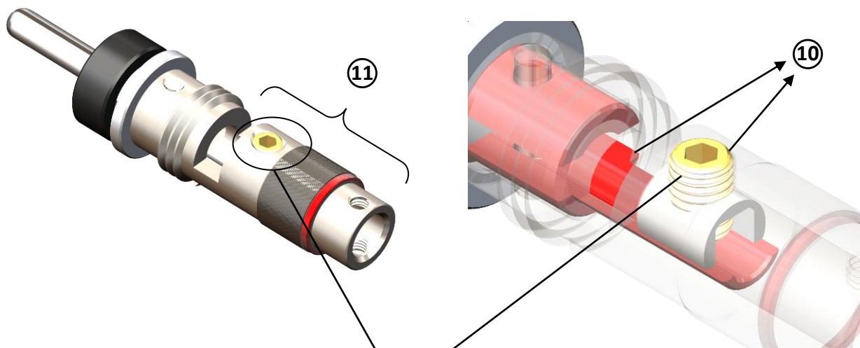
Copper alloy set screw (H2.0) 2
